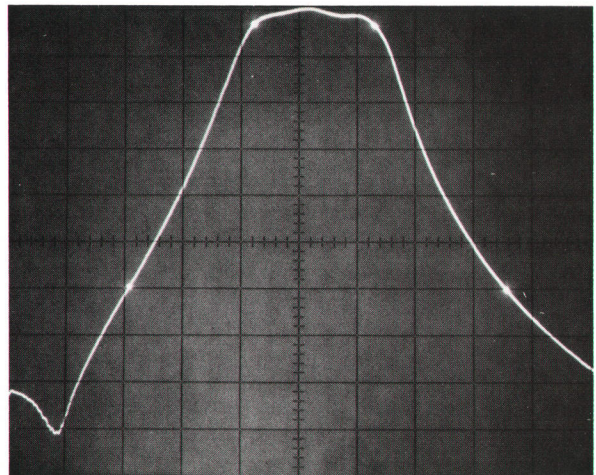
Intensity markers indicate where measured quantity crosses high and low limits stored in processor.
