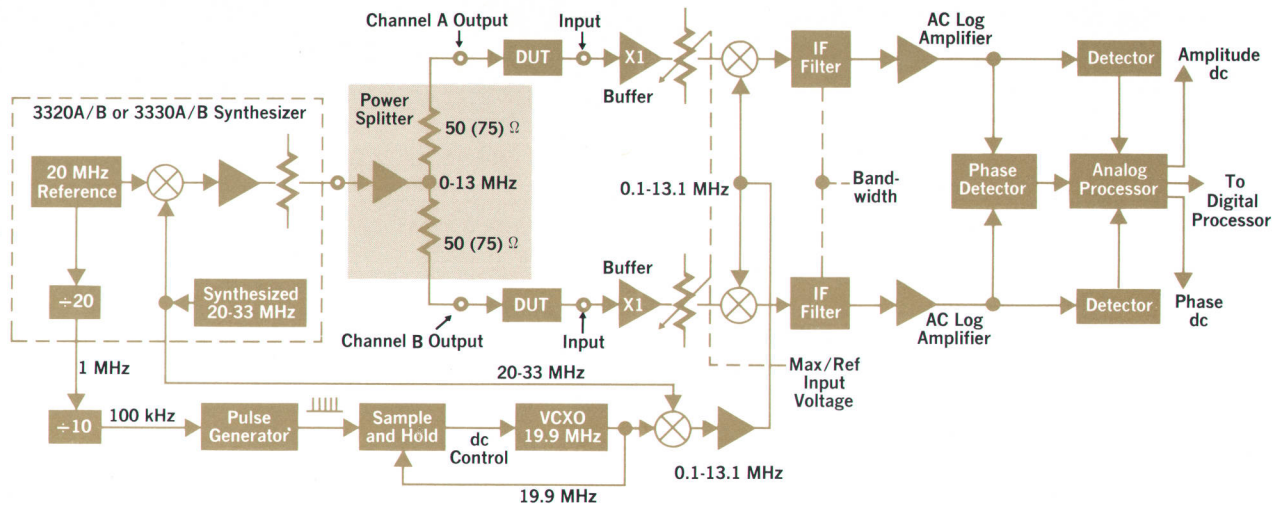
A. Simplified block diagram of Network Analyzer includes pertinent sections of Frequency Synthesizer. Device under test (DUT) connects between channel output and input.
